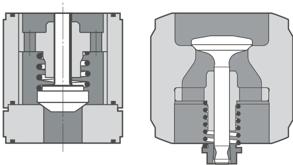
Cone valve
